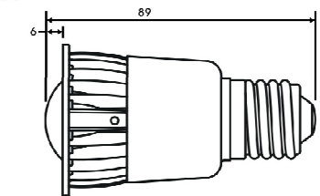
TRISTAR-E27-L
